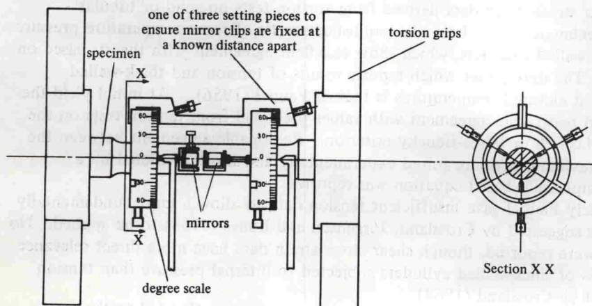
Figure 2. General arrangement of torsionmeter for measuring small and large strains.
