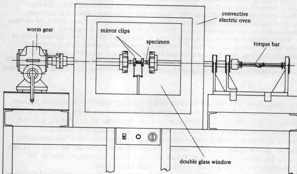
Figure 1. General arrangement of torsion testing machine for elevated temperatures.
